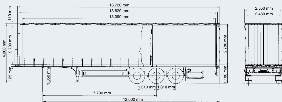
S.CS 24/L – 13.62 CEB – three-axle semitrailer with curtainsider tensioned tarpaulin design
